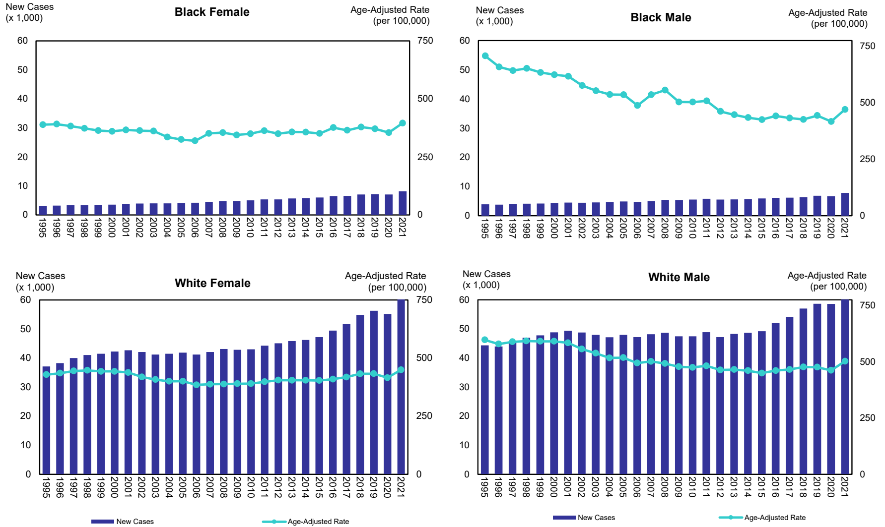
Figure 3. New Cases and Age Adjusted Incidence Rates for All Cancers by Sex and Race, Florida, 1995-2021
